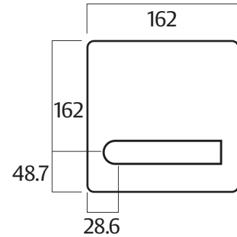
Artefact - Radiused Corners (162 X 162 X 2mm)
