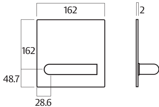
Artefact - Square Corners (162 X 162 X 2mm)
